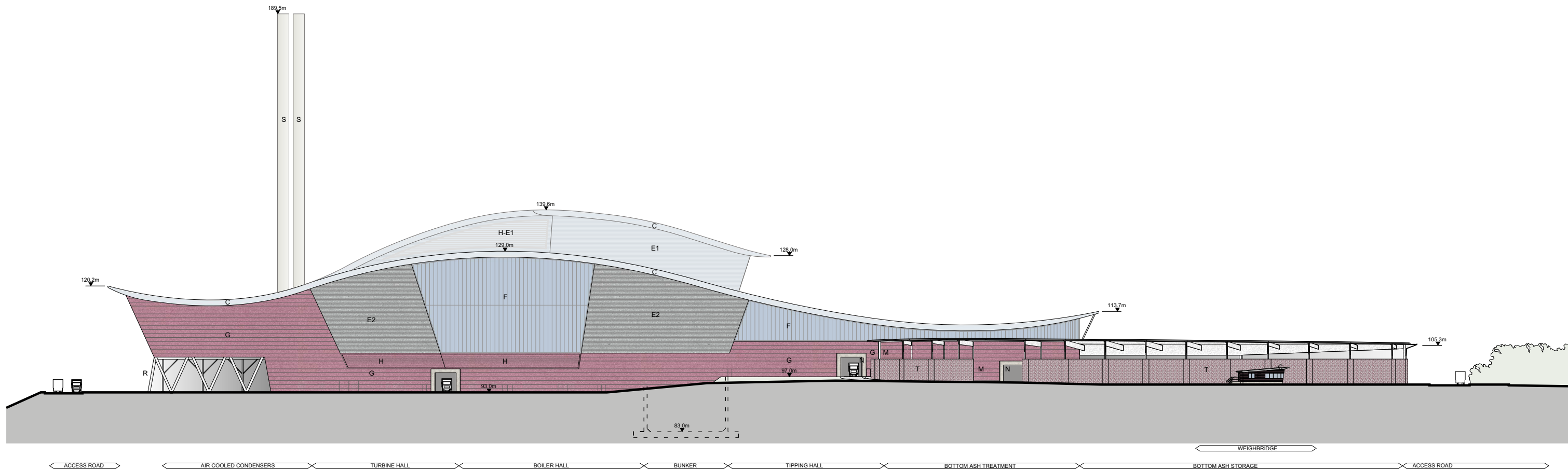
EAST ELEVATION
