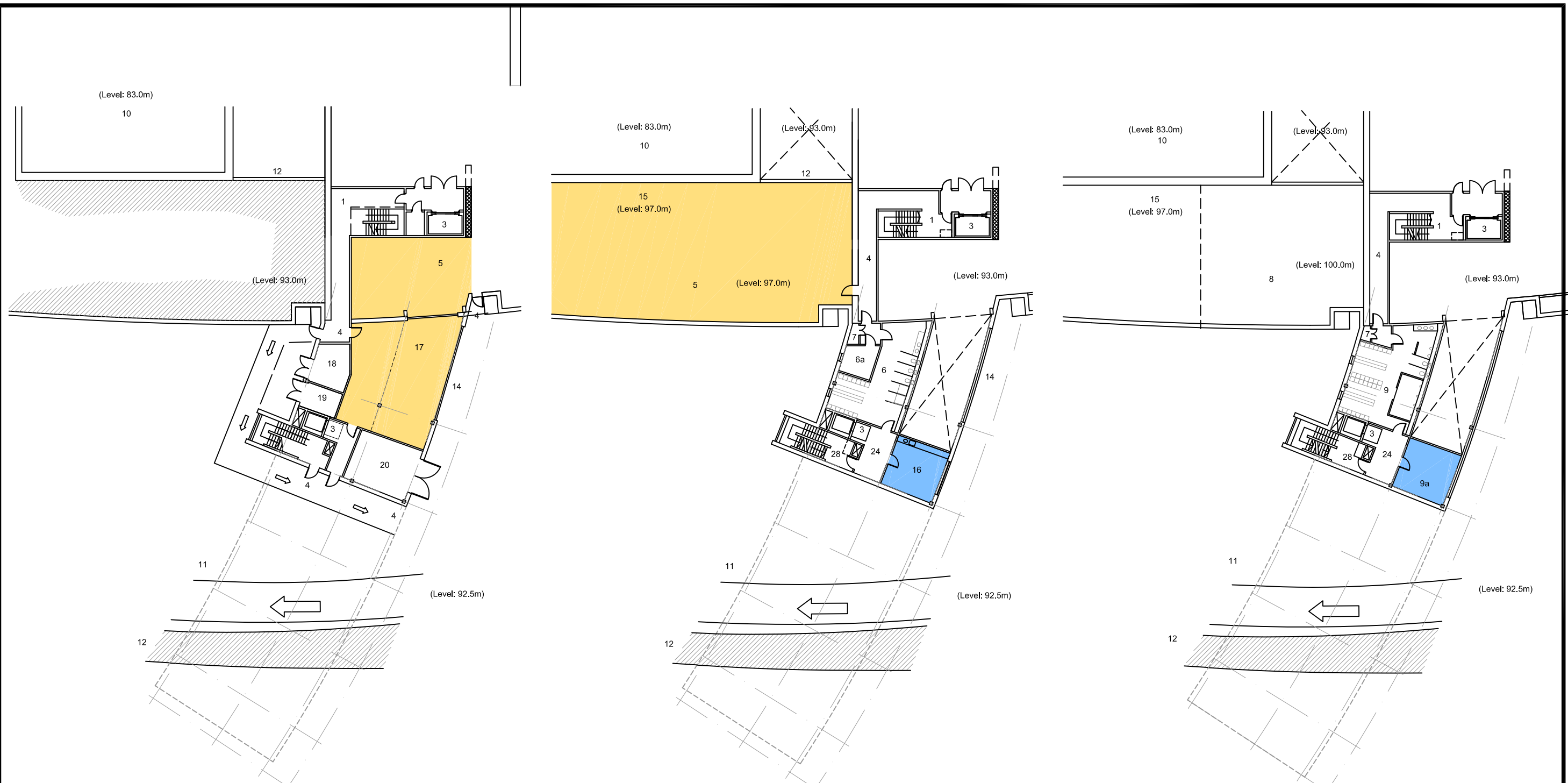
LEVEL 93.0m PLANT ROOMS / PARTS STORE
